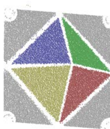
Figure 27: Derived objects, such as building corners, are located within the scan data separately for each face of the scan and compared against the location of the corner found by the Leica TS30. The plates are built and measured in advance of mounting so the relationship between the total station prisms and the corner is known in advance.
