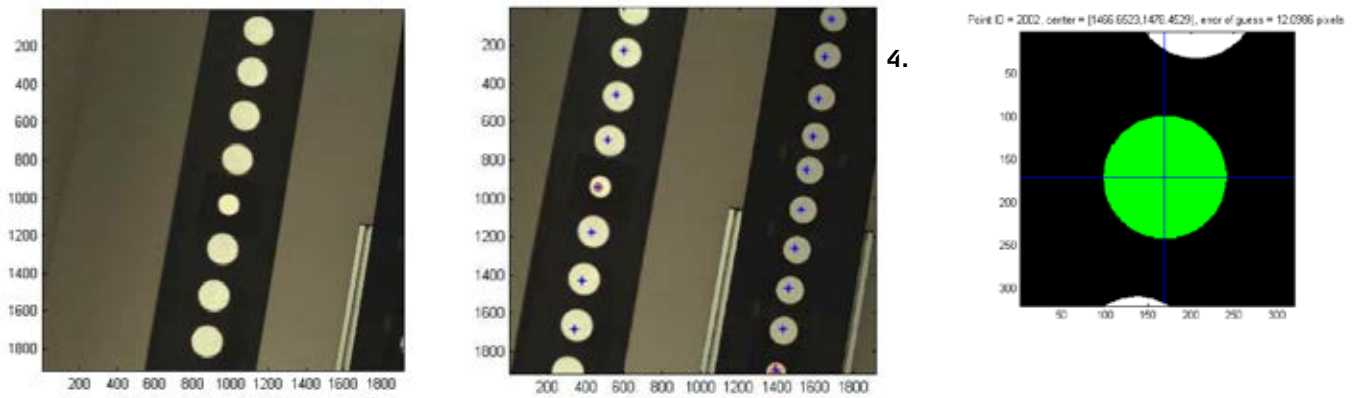
Figure 20: Images from a Leica ScanStation C10 scanner as viewed in MATLAB ® . MATLAB ® has drawn on the image guess locations of the target centres using an approximate camera model. These guess locations are used to solve the target correspondence problem, and are generally off by a gross amount such as 15 or 20 pixels. This is close enough to prepare the matches.
