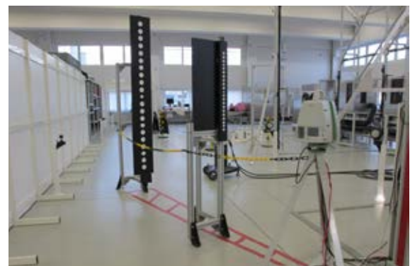
Figure 19: A view of the camera calibration stand. Two sets of targets are placed in front of the scanner and are both imaged and scanned.
